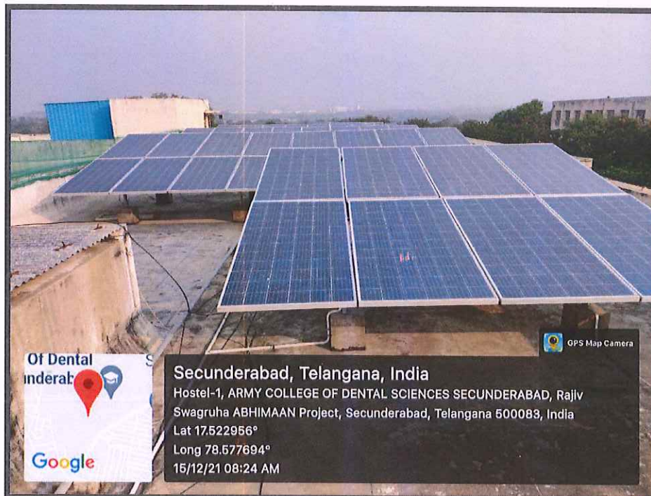
Fig-2: 25 KW solar roof top power grid
